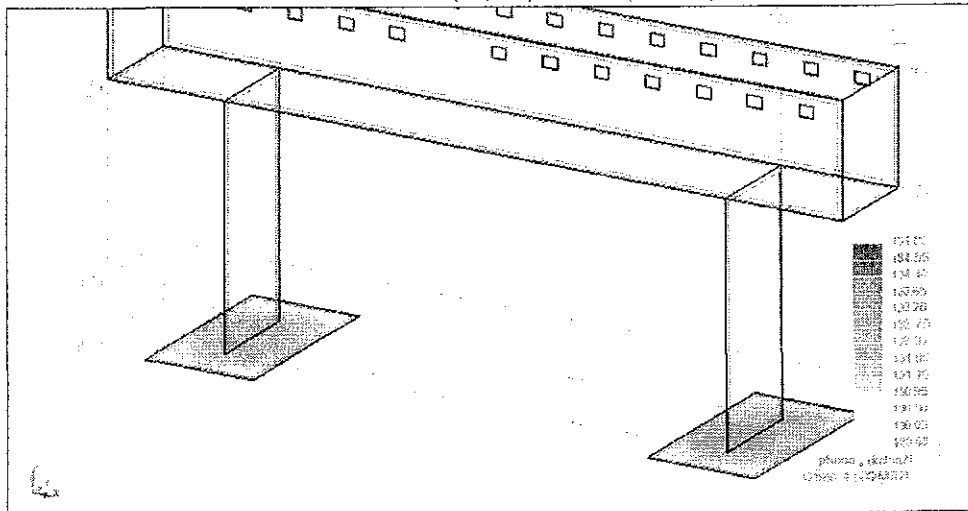
View - Soil reaction. (kN/m2) Cases: 4 (COMB2) 1
